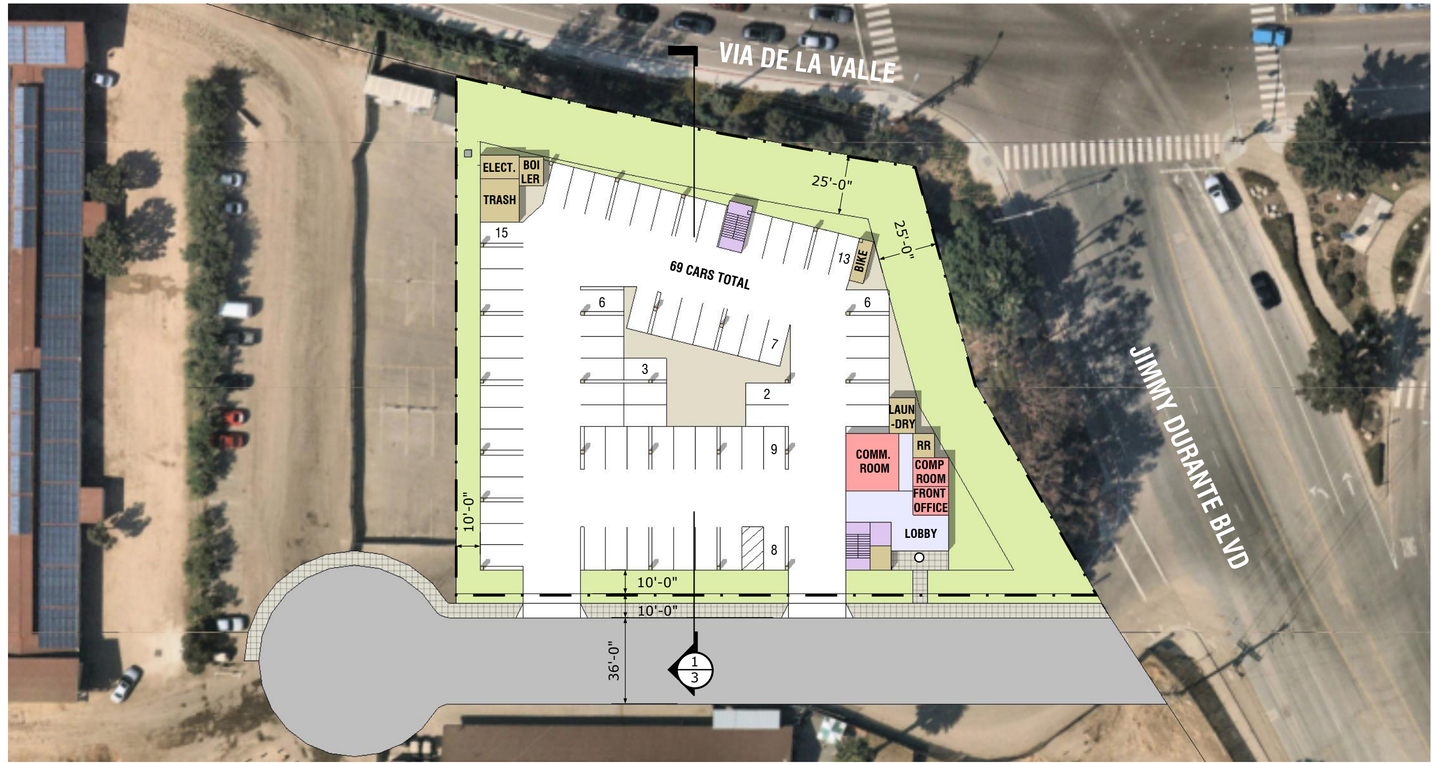
SITE PLAN
