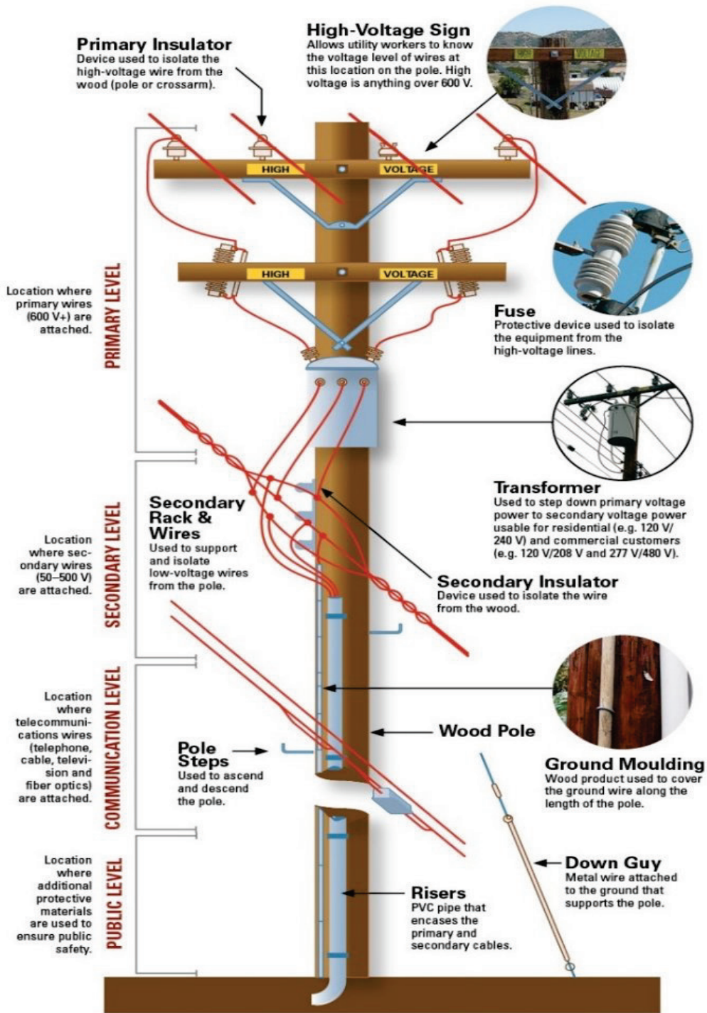
Figure 1: Utility pole diagram 1
