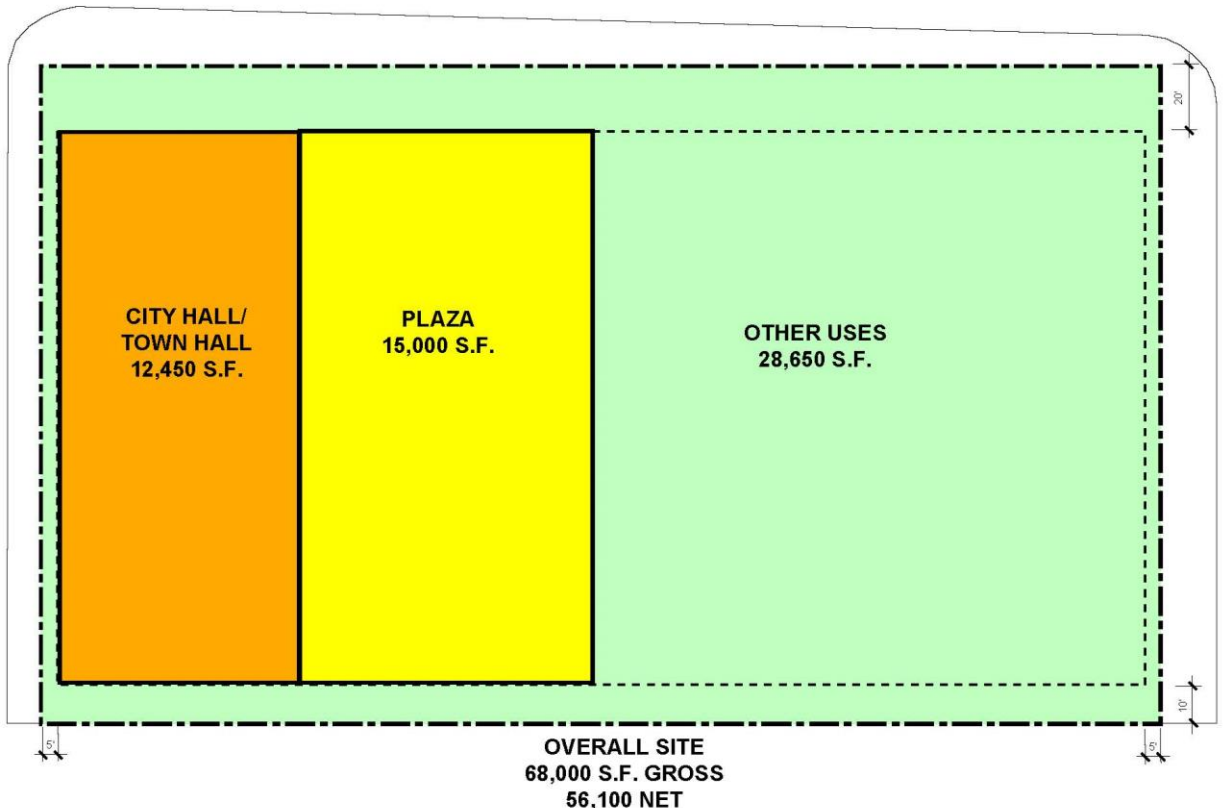
CIVIC CENTER SPACE DIAGRAM PLAN B - CIVIC PLANNED FOR FUTURE OPTIONS WITH BELOW-GRADE PARKING
