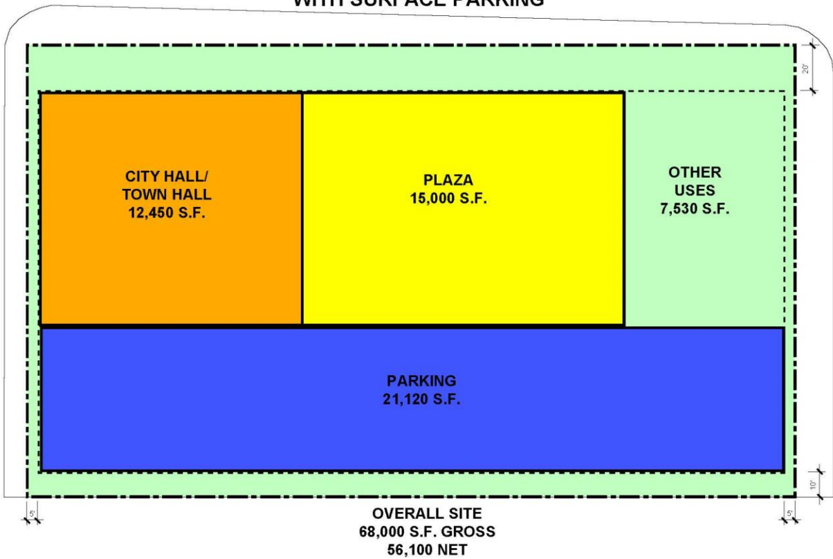
CIVIC CENTER SPACE DIAGRAM PLAN A - CIVIC ONLY WITH SURFACE PARKING
